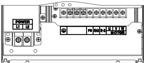
4.0-11kW Main circuit terminal
