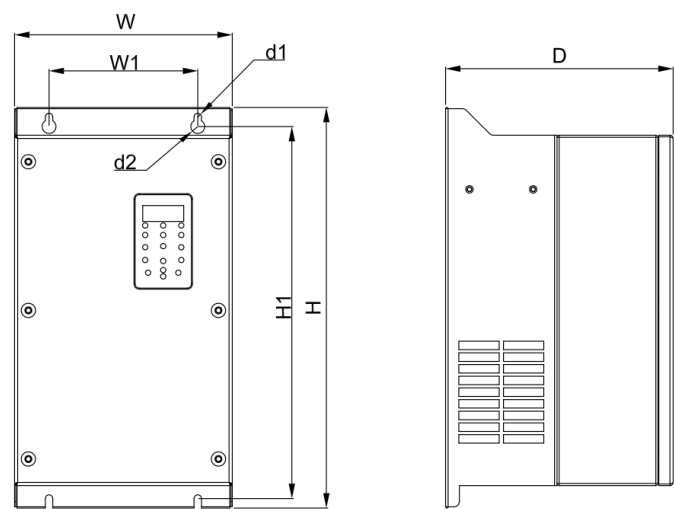
Dimension Drawing
