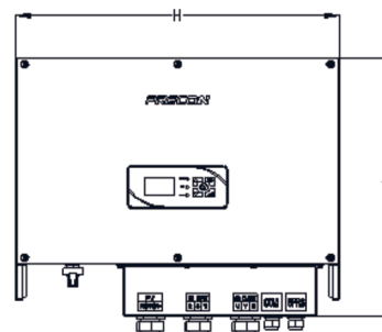
Schematic diagram of product size ( \geq 30\text{kW} )
