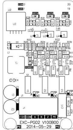
Fig.C-2(b)EXC-PG02
