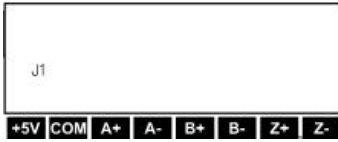
Fig.C-3(a)EXC-PG01 terminals
