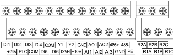
Fig.2-10b Control circuit terminals(>2.2KW)
