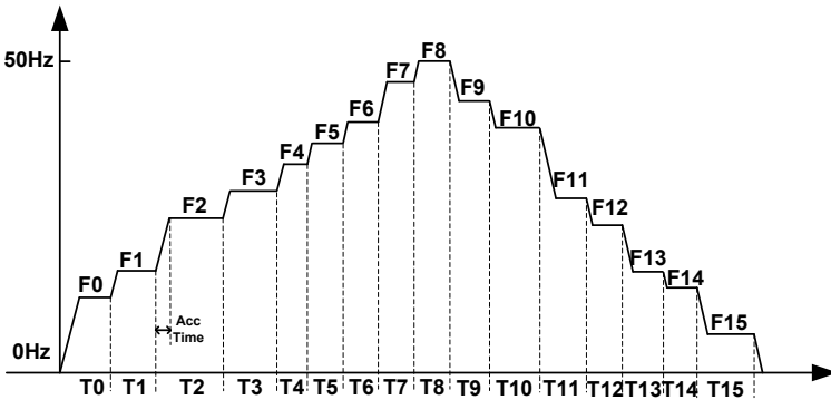
Figure 3-2 linear mode running diagram
