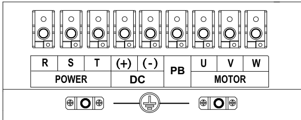
Fig.1-10 45~90kW Schematic of main circuit terminals
