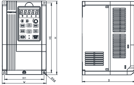
Fig 1-4 4~22kW Wall installation diagram
