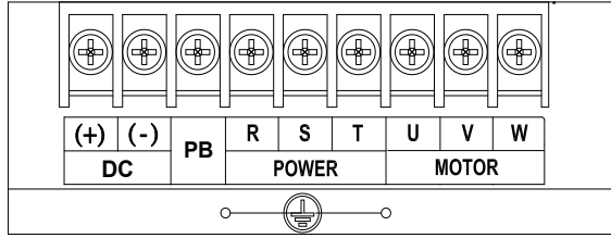
Fig.1-9 30~37kW Schematic of main circuit terminals
