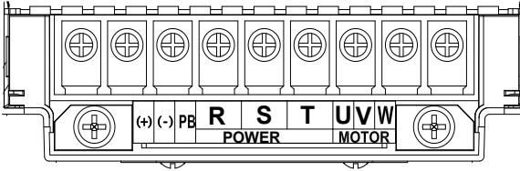
Fig.1-7 4~5.5kW Schematic of main circuit terminals
