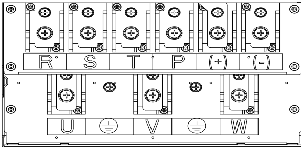
Fig.1-11 110~132KW , 250~280KW ,315~355KW Main Circuit Terminals
