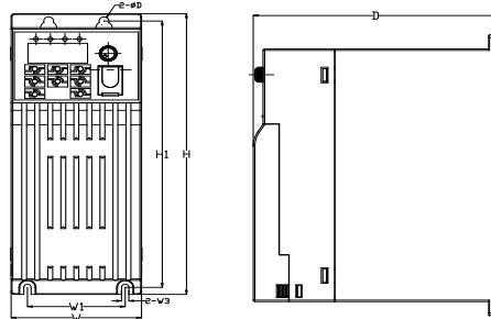
Fig 1-3 0.7~2.2kW Wall installation diagram
