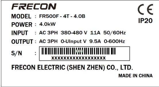
Figure 1-1 Nameplate Information
