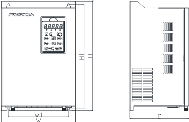
Fig 1-5 30~355KW Wall installation diagram
