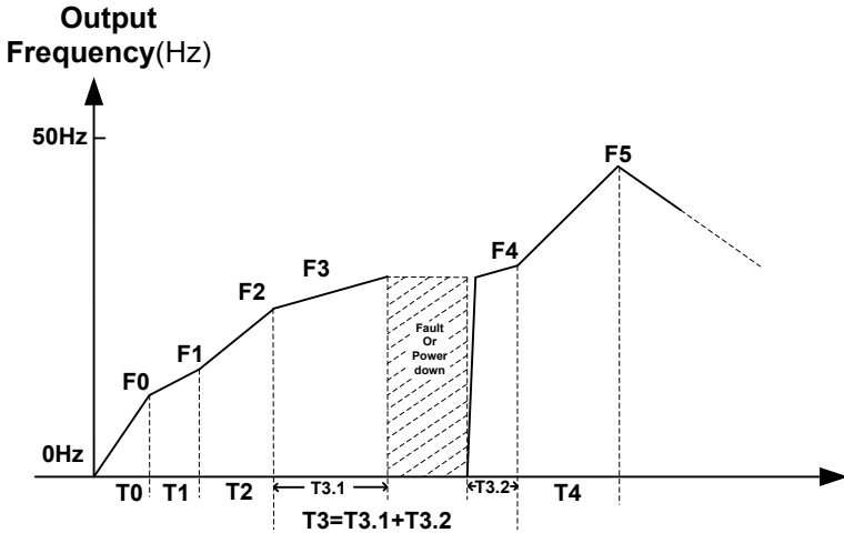
Figure 2-6 power-off memory function diagram
