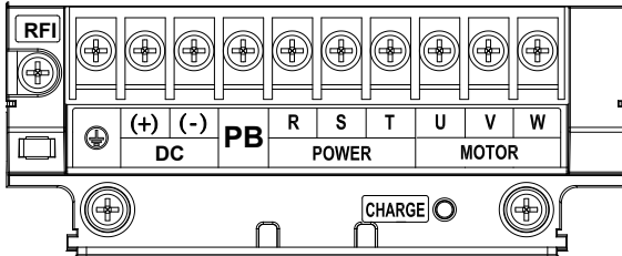
Fig.1-8 7.5~22kW Schematic of main circuit terminals
