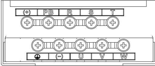
Fig.1-6 0.7~2.2kW Schematic of main circuit terminals
