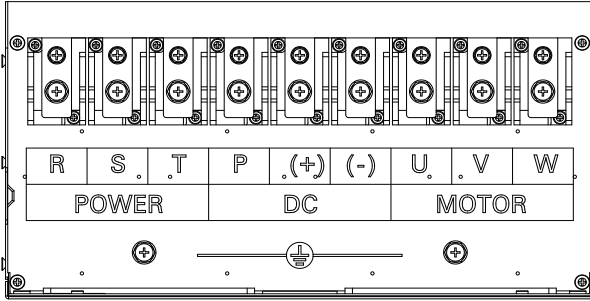
Fig.1-11 160~220KW Main Circuit Terminals
